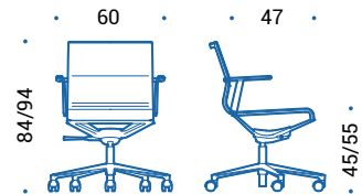
ATK.351T | swivel chair, height adjustable, tilting mechanism, backrest handle and armrests in aluminum with cover in plastic
